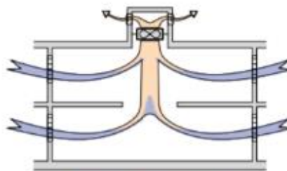
Figure 8 : ventilation hybride
